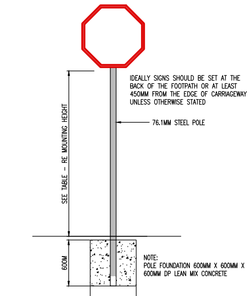
TYPICAL MOUNTING ARRANGEMENT FOR SIGNS IN VERGES AND FOOTPATHS INCLUDING FOUNDATION DETAILS SCALE 1:50
